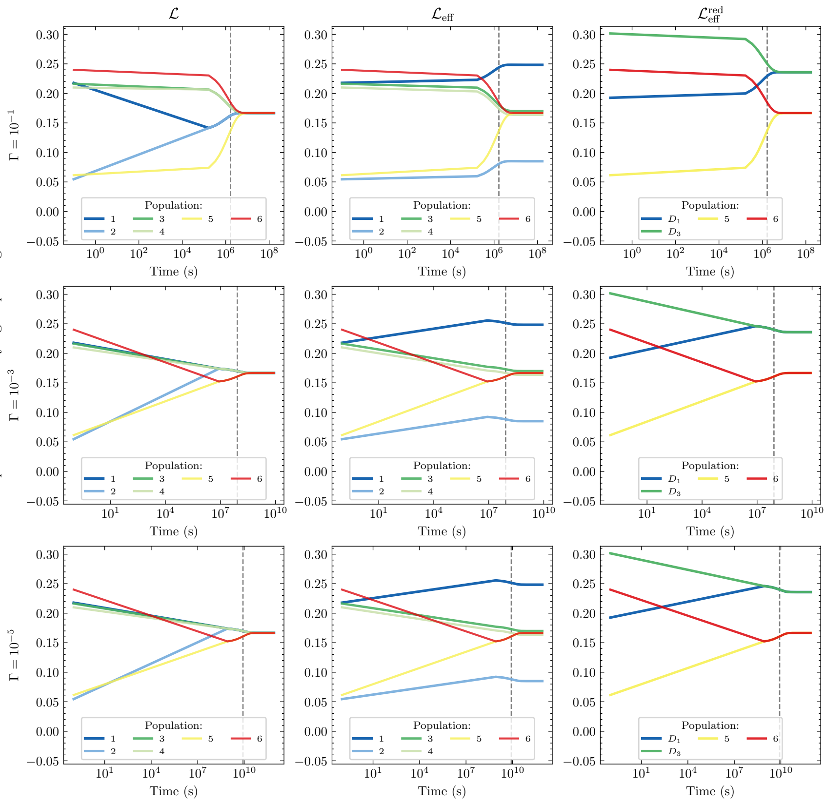
Time Evolution of Site Populations under \mathcal{L} , \mathcal{L}_{\text{eff}} , and \mathcal{L}_{\text{eff}}^{\text{red}} n_d=2 ; n_\epsilon=2 ; J = 10^{-1} ; \epsilon = 10^{-4}
